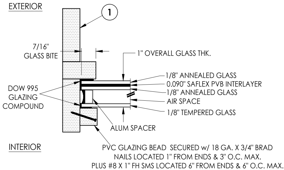
G1 GLAZING DETAIL Transom
